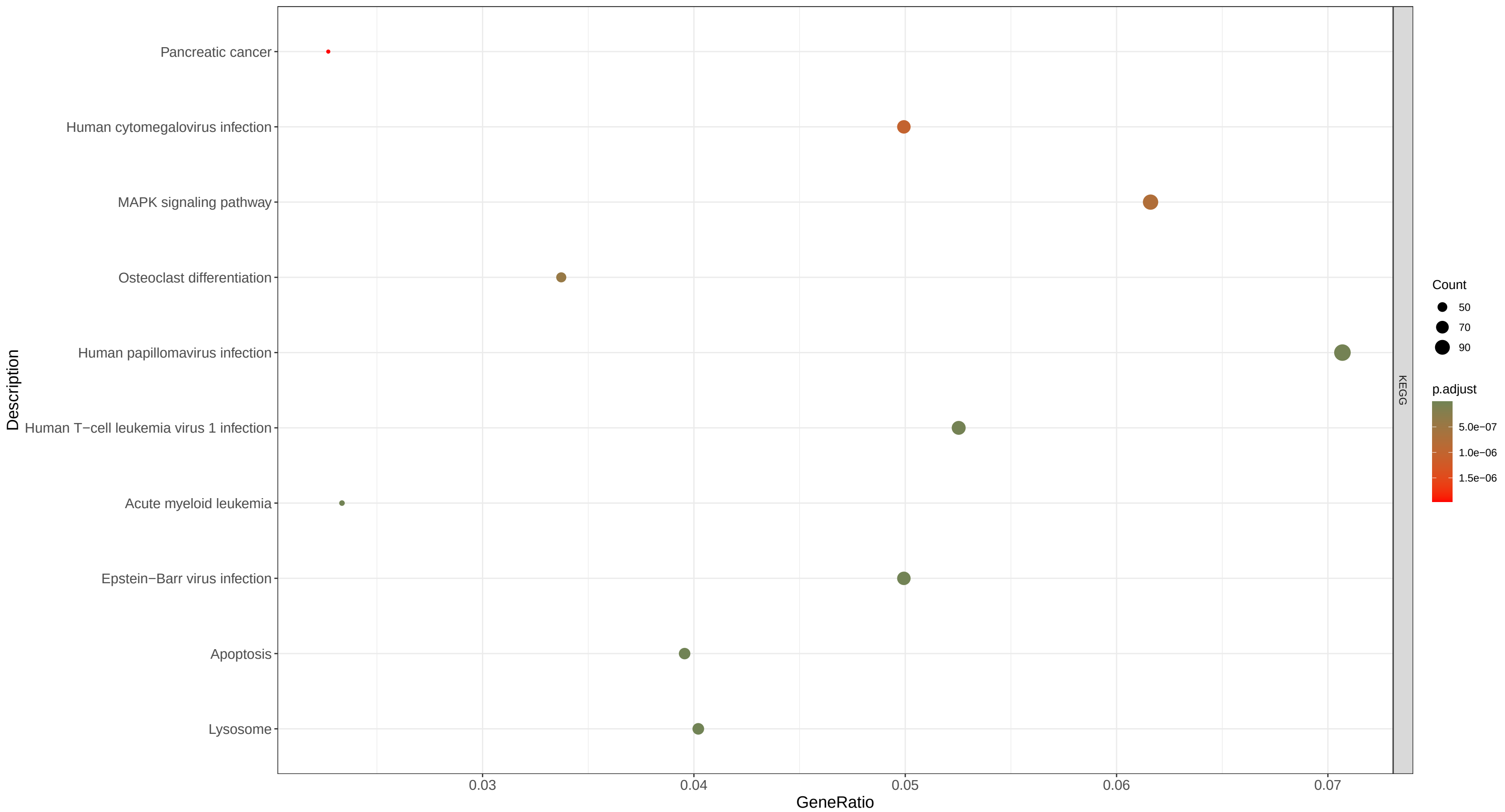
RABC Enriched KEGG_RABC1
